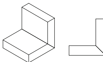
MITER UV GLUE SEAM
