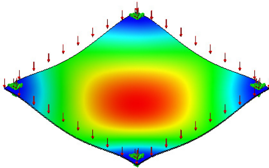
Figure 5. Point-support deflection diagram
